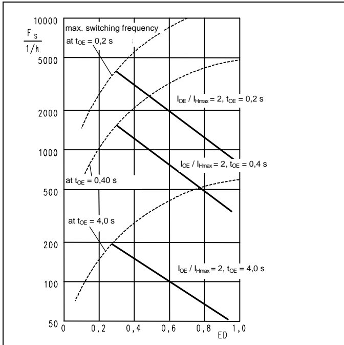
Diagram 1: Permissible maximum switch frequency Rectifiers installed in switch cabinets with a minimum distance of 30 mm to adjacent units.
