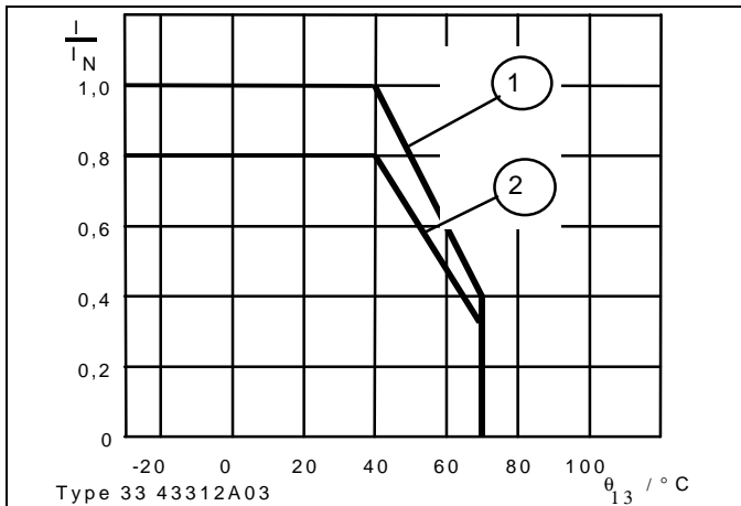
Diagram 2: Admissible current load at ambient temperature ① distance between 2 devices minimum 30 mm ② distance between 2 devices below 30 mm
